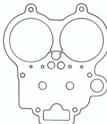
7428 42 DFC-1 45 DFC
