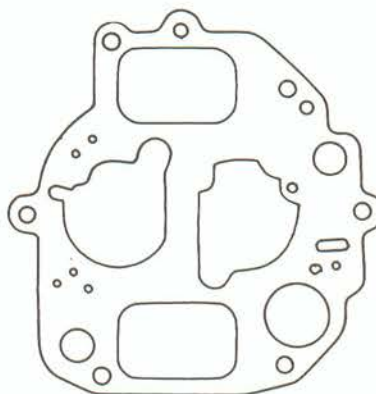
7795 26/32 CSIC
