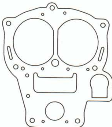
7691 Opel Manta
