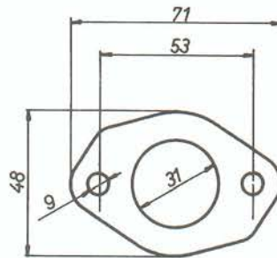
7282 32 PDIST
