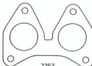
7353 Fulvia Rally
