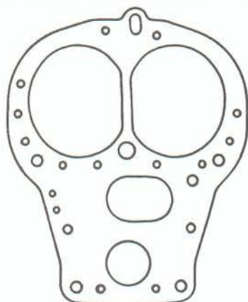
7367 35 SDID
