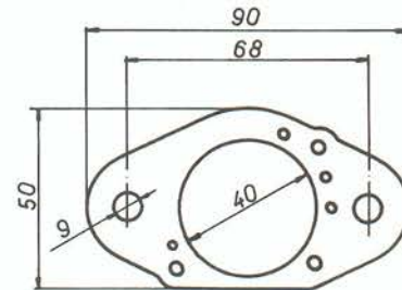
7253 36/40 PDSIT BMW 2000
