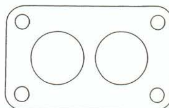
7996 34 DMTR Citroën CX 2000
