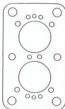
7542 32 TDID Ford Taunus Granada
