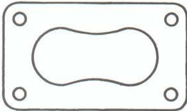
7360 32/35 DDIST
